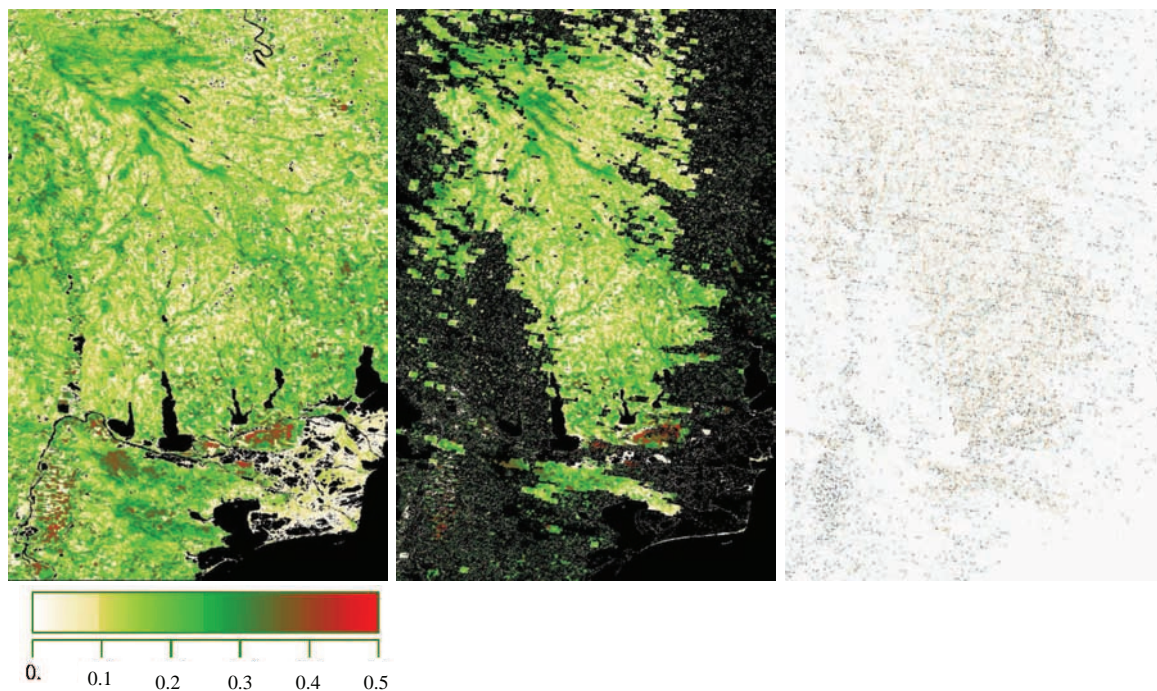
FIGURE 1. Maps of FAPAR values and differences over Romania for the 2 nd of May 2010. Left panel: JRC calculations using the entire swath. Middle panel: VITO products where the second day has been selected in the 10-days product. Right Panel: Difference between the two products
