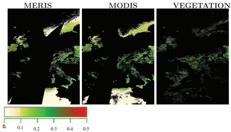
FIGURE 7. Same as Fig. 6. but for the 8 of MAY 2010.
