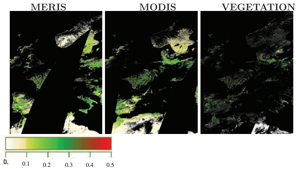
FIGURE 6. Daily FAPAR maps over Europe from MERIS (ESA), MODIS(JRC) and VGT (VITO) instruments for the 2 nd of MAY 2010.
