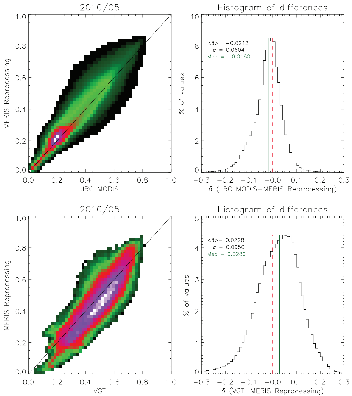
FIGURE 8. Scatter-plots and histogram of differences between daily values from MODIS TERRA (top panel) and VGT (bottom) versus MERIS instruments.
