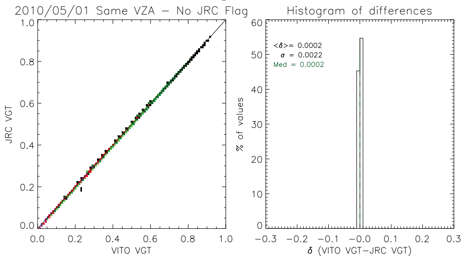
FIGURE 4. Same as Figure 3 for the same SZA.
